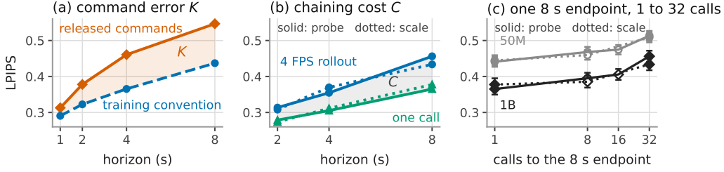
Figure 1: (a) The command error K is the band between the 1B model’s 4 FPS rollout under the released commands and under the training convention; its growth from 2 to 8 s is a third of the released curve’s rise (post hoc; confirmation cohort, 200 trajectories). (b) The chaining cost C is the band between the same model’s corrected 4 FPS rollout and a single call to the same moment; its growth from 2 to 8 s is two fifths of the corrected rollout’s rise on the probe cohort (solid lines, band) and a sixth on the scale cohort (dotted), 150 trajectories each (post hoc). (c) The 8 s endpoint reached with corrected commands in 1, 8, 16 (probe cohort only) and 32 calls by the 1B and 50M models on both cohorts, on a logarithmic axis; the 8- and 16-call rollouts (open markers) condition on generated frames 1 s and 0.5 s apart, a spacing the model never saw (Section 3.1). Bars are 95% trajectory-bootstrap intervals of each mean, not of paired differences; (a) and (b) show means only.
