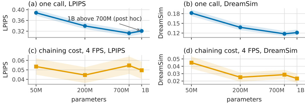
Figure 4: On the scale cohort, the one-call error (top) falls on LPIPS from 50M to 700M and is higher at 1B than at 700M (post hoc), while the 4 FPS chaining cost (bottom, on its own axis) shows no detectable trend on LPIPS (left) and a decrease on DreamSim (right). Values are means over 2, 4 and 8 s against the number of parameters, with 95% trajectory-bootstrap bands from one joint resampling; with one checkpoint per size, the bands cover evaluation variance only. The 700M and 1B bands overlap although their paired difference is resolved on LPIPS (post hoc); it is not resolved on DreamSim). The bottom row’s axes span a narrower range than the top row’s.
